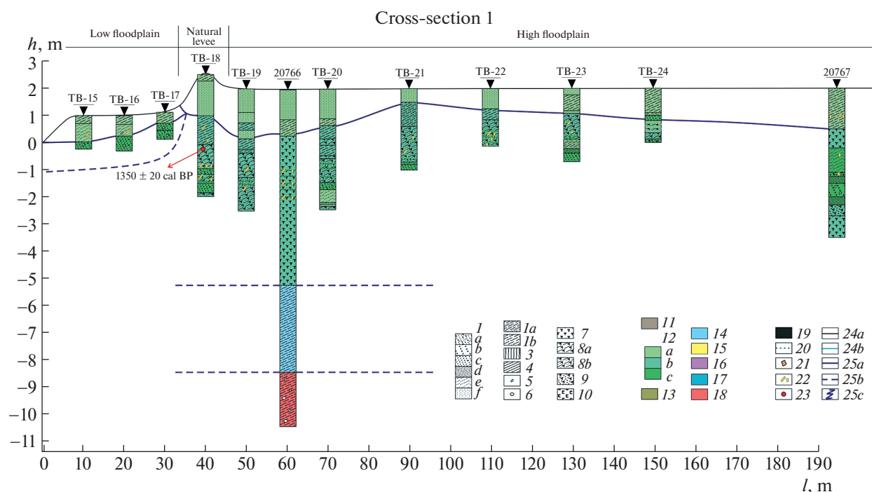
Fig. 4. Toropa river valley cross-section 1. Texture: 1 – sand ( a – diamicton, b – very coarse, c – coarse, d – medium, e – fine, f – very fine); 2 a – sandy loam; 2 b – clayey loam; 3 – silt; 4 – clay; 5 – gravel; 6 – pebble; 7 – peat; 8 – peat ( a – sandy loam, b – clayey loam); 9 – sand; 10 – gyttja. Genesis and age of deposits: 11 – alluvial fan Q4; 12 – alluvium Q4 ( a – overbank, b – swampy overbank, c – channel); 13 – marsh Q4; 14 – lacustrine Q4; 15 – colluvium Q4; 16 – glaciofluvial MIS 2; 17 – limno-glacial MIS 2; 18 – till of the Valdai glaciation. Other designations: 19 – cultural layer of the IX–XI c.; 20 – presumed boundaries of the cultural layer of the IX–XI c.; 21 – archaeological artifacts of the IX–XI c.; 22 – plant remains; 23 – dates ^{14}\text{C} , cal. years BP; 24 – topography of ( a – landscape, b – lake bottom); 25 – boundaries ( a – precise, b – imprecise, c – facial).
