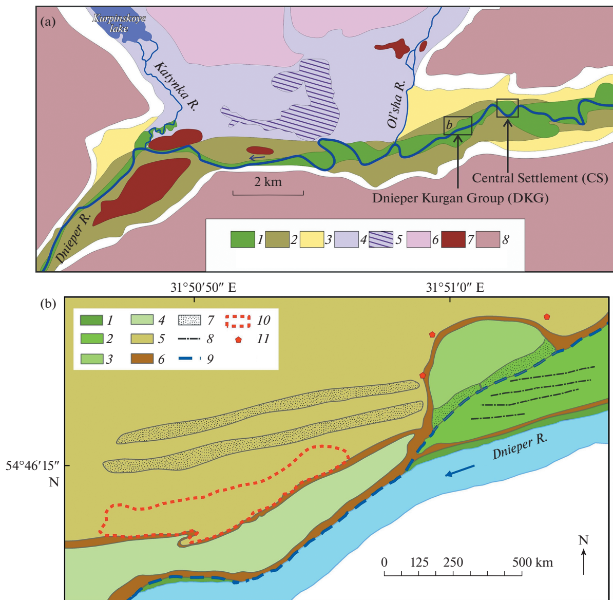
Fig. 2. (a) – Geomorphological map of the upper Dnieper valley: 1 – 5–9 m floodplain terrace (Q4); terraces: 2 – 10–13 m (Late Glacial – Early Holocene); 3 – 13–15 m (MIS 3–4); 4 – alluvial valley bottoms reworked by glaciofluvial processes (LGM); 5 – glaciofluvial ridges (eskers), LGM; 6 – morain terrain of the Late Valdaian glaciation (MIS 2); 7 – erosion remnants composed of glacial tills of different ages; 8 – partly reworked morain/glaciofluvial terrain of the Moscovian glaciation (MIS 6). From (Panin et al., 2014) with supplements. (b) – Geomorphological map of the right bank of Dnieper at the Dnieper Kurgan Group: 1 – low floodplain, 2 – 4–6 m floodplain (300–200 BP), 3 – 4–5 m floodplain (2.5–2 ka BP), 4 – 8–9 m floodplain (11–8 ka BP), 5 – terrace, 6 – erosional slopes, 7 – levees, 8 – floodplain ridges, 9 – the right bank of Dnieper river in IX–XI c. AD, 10 – the main mounds area, 11 – separate mounds. Based on geomorphological survey. Note: elevation of river terrace are related to the Dnieper valley and expressed in meters above the river at the typical low-water stage.
